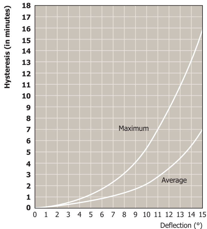
Series 20 - Max. \theta \pm 7.5^\circ
